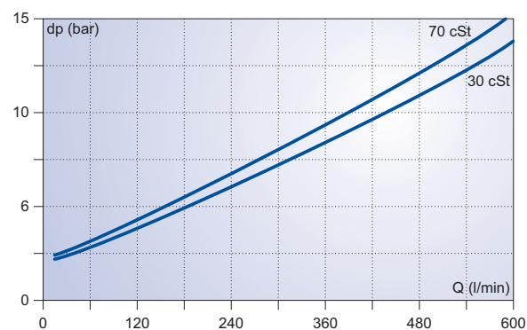
Q = 12 ... 600 l/min
